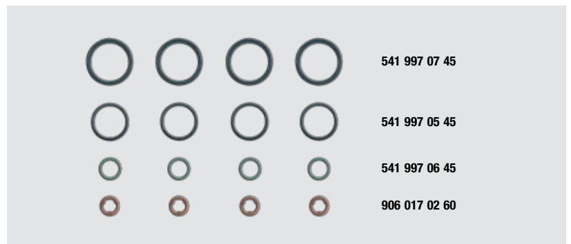
Fig. 1_OM 904 / OM 924, injection nozzle set 15-31357-02
