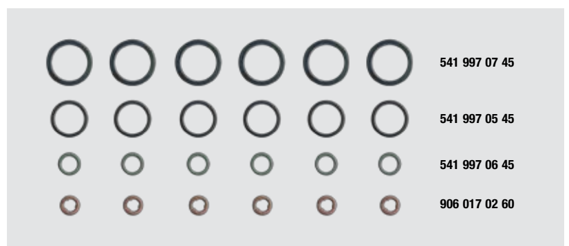
Fig. 2_OM 906 / OM 926, injection nozzle set 15-31357-03
